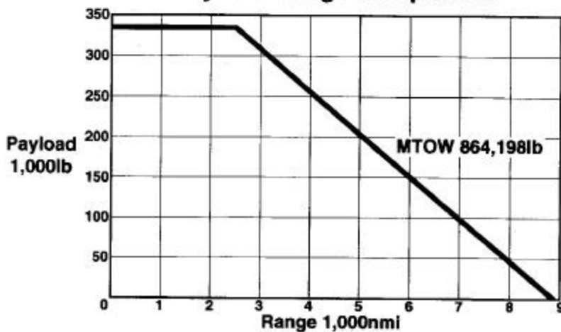
Antonov AN-124 Payload-Range Comparison
